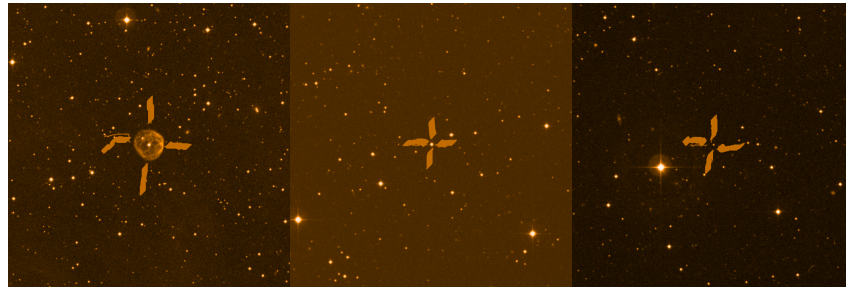
(a) NGC 7094
