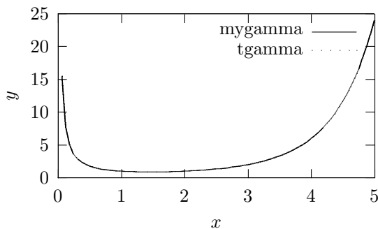
Figure 1: Nemes formula (2) via gnuplot "latex" terminal.
