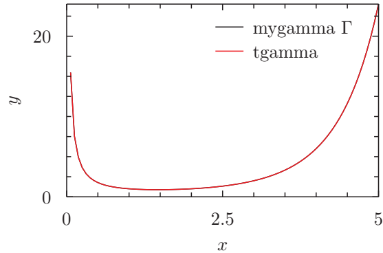
Figure 2: Nemes formula (2) via pyxplot "pdf" terminal.
