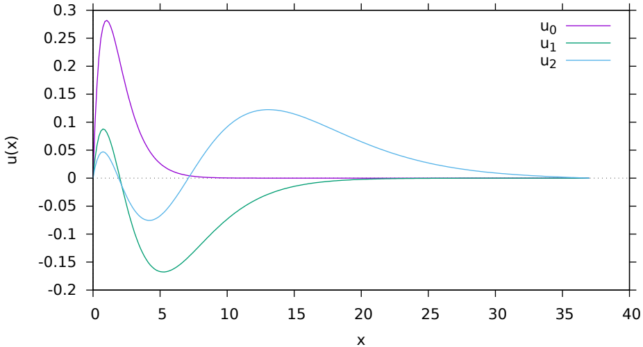
eigen-functions
