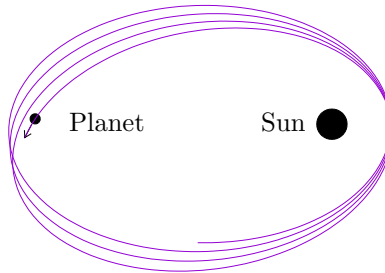
Figure 1: Aphelion shift of a planet orbiting a star.
