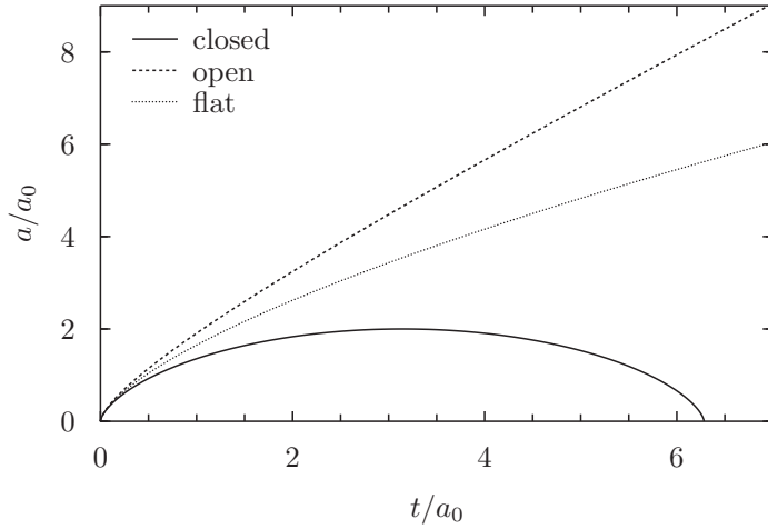
Figure 1: The scale a(t) of a mass-dominated Friedman universe as function of time t for the open, closed, and flat geometries.
