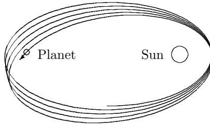
Figure 1: Apse shift of a planet orbiting a star.
