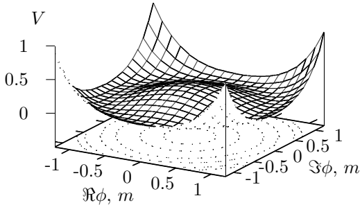
Figure 1: ‘‘Mexican hat’’ potential (2) in arbitrary units as function of the real, \Re\varphi , and imaginary, \Im\varphi , parts of the complex scalar field \varphi .
