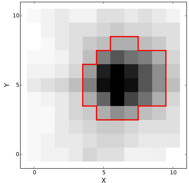
FIG. 1.— Pixel mask for K2-39. The grey scale indicates the electron count, going from black (high) to white (low). The red line encircles the aperture used to generate the photometry, which includes all pixels with counts more than six times the median flux value.
