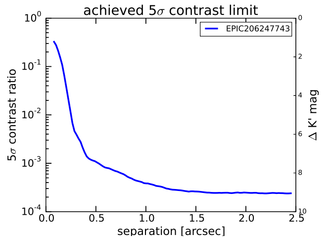
FIG. 4.— Adaptive optics image using the Subaru telescope. The orientation is North-up and East-left, as in Figure 3. In the top figure, the image for K2-39 is shown. The middle figure shows a standard star (FS151) observed during the same night, which has a slightly non-circular shape, suggesting a degraded AO performance. The bottom image shows the 5\sigma contrasting ratio the image provides.
